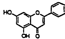
CHRYSIN
